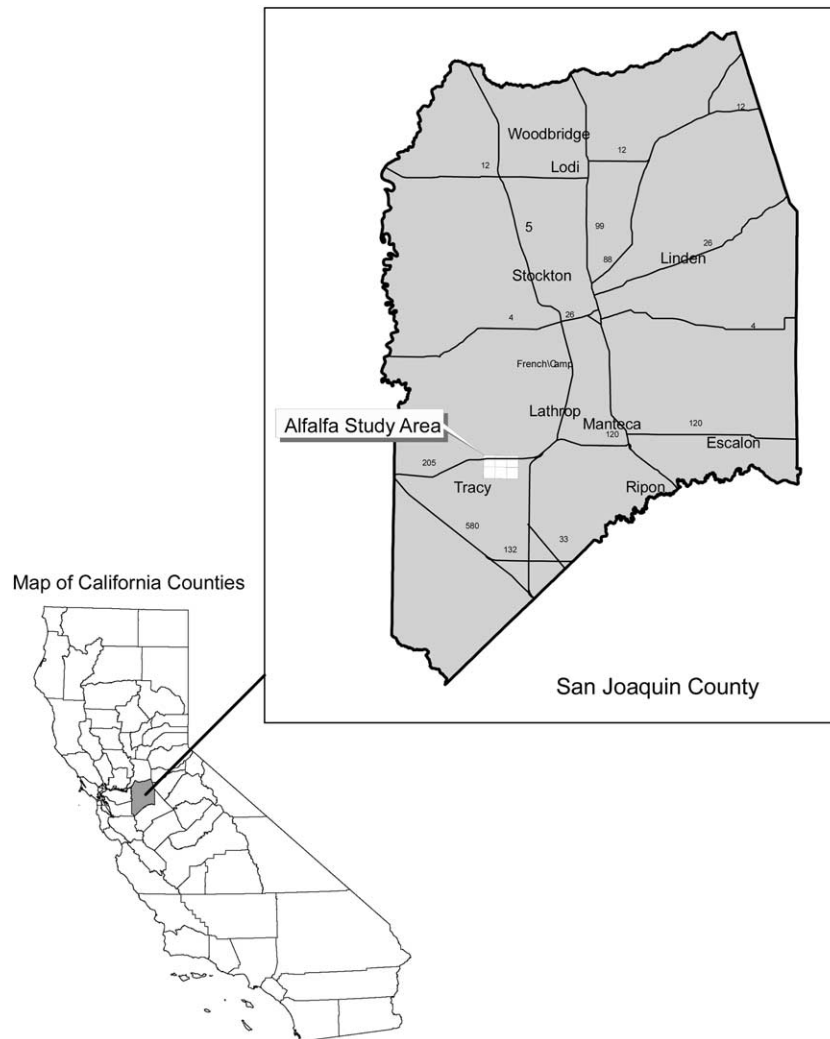
Fig. 1. Location of the alfalfa study site near Tracy, CA.
