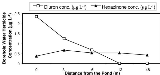
Fig. 6. Concentration of diuron and hexazinone measured in ground water samples obtained along a transect at increasing distances from the holding pond.
