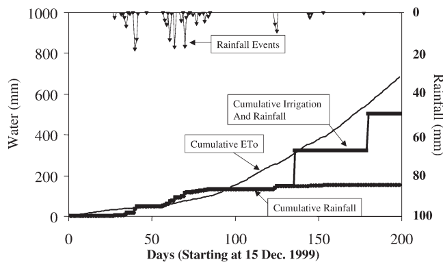
Fig. 3. Comparison of cumulative reference evapotranspiration ( ET_0 ) to cumulative rainfall and to cumulative rainfall plus irrigation water volumes as indicated by the bottom and left axes. Specific rainfall events and water depth are indicated on the top and right axes.
