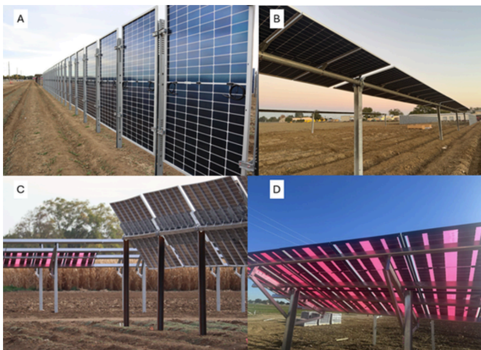
Figure 4. Four different agrivoltaics technologies are simultaneously utilized to assess agrivoltaics feasibility at UC Davis: (A) 50 KW vertical solar system with bifacial panels; (B and C) two 50 KW systems utilizing two different single-axis racking system along with bifacial solar panels; and (D) 50 KW fixed-tilt with spectral-selective solar panels (Images were provided by Dr. Majdi Abou Najm at UC Davis).
