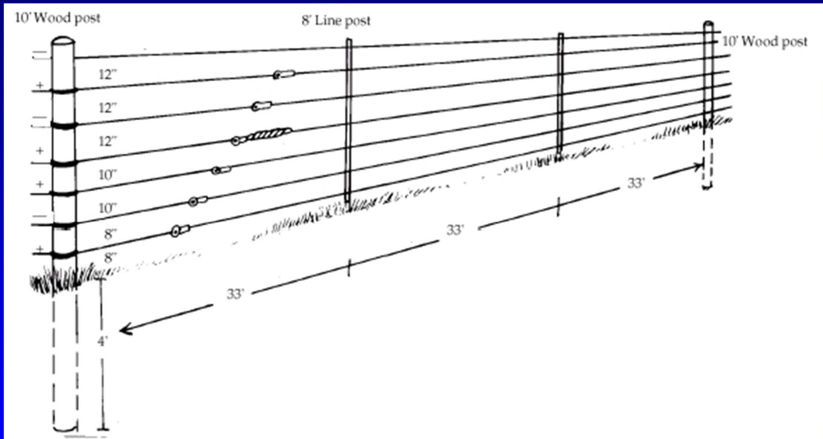
7-wire vertical electric fence
