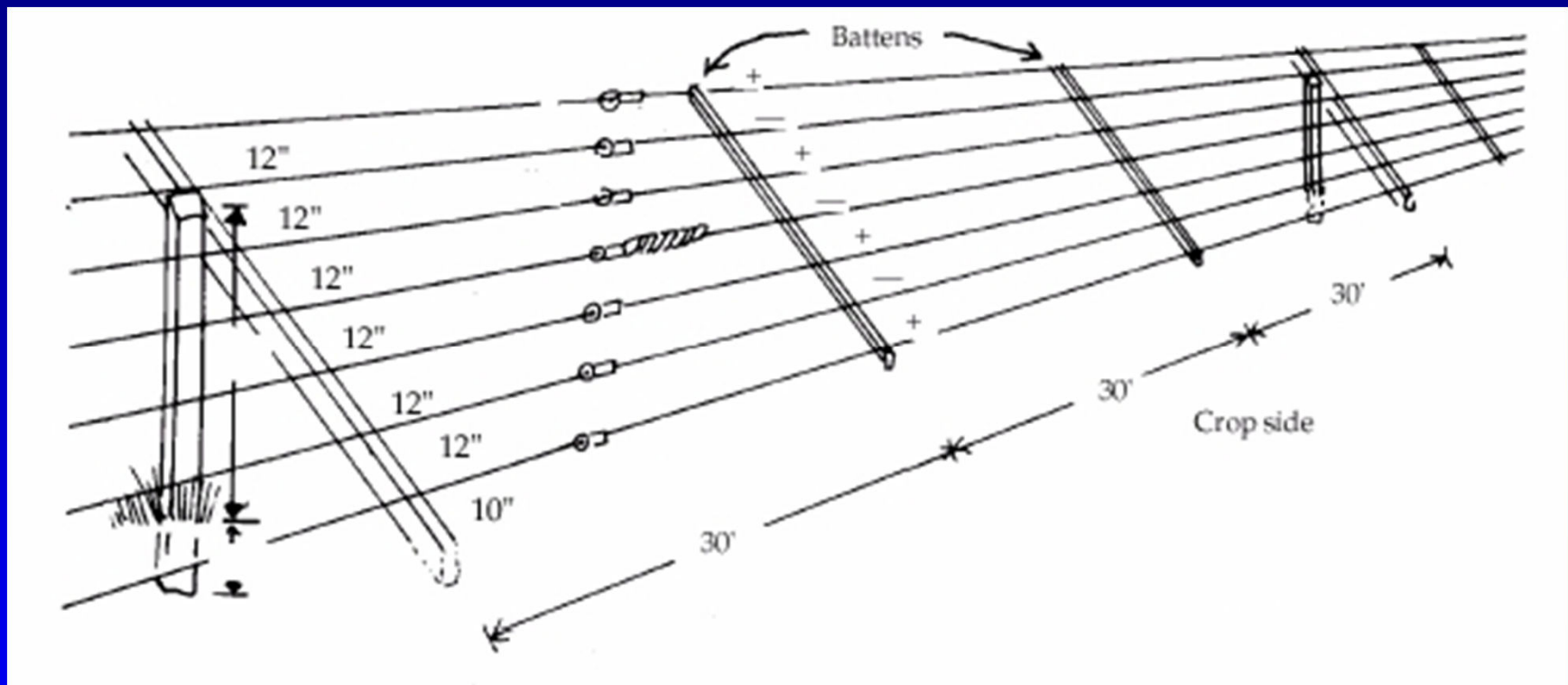
Slanted 7-wire deer fence
